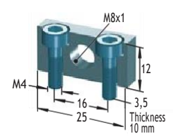
Mounting Block
